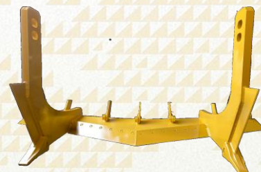
Double Tyne "V" for row planted and larger stump diameters that pin in the outer Ripper Pockets. Width up to 7.5m
